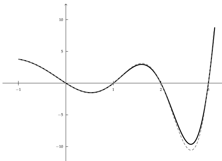
Figure 3. The gray color curve represents the function in the left hand side in (54) for n = 100 and black curve is the limiting function.
