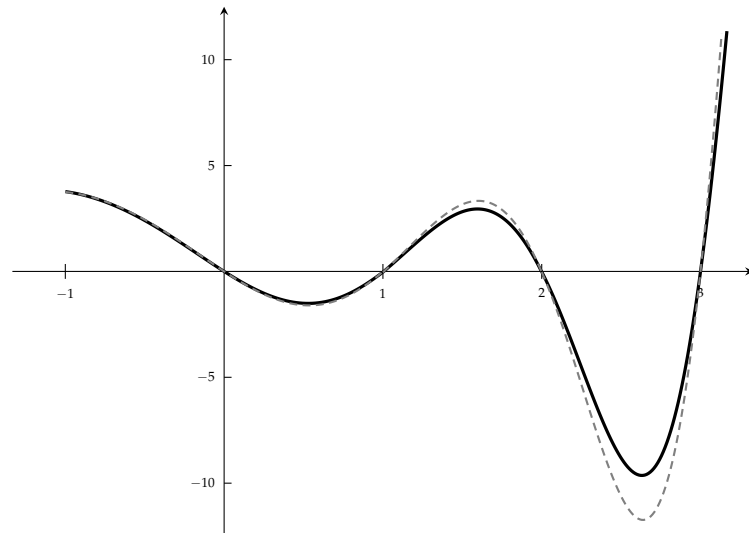
Figure 1. The gray color curve represents the function in the left hand side in (54) for n = 50 and black curve is the limiting function. Data: \beta = 7, c = 1/5, \lambda = 10^{-21} and j = 2 .
