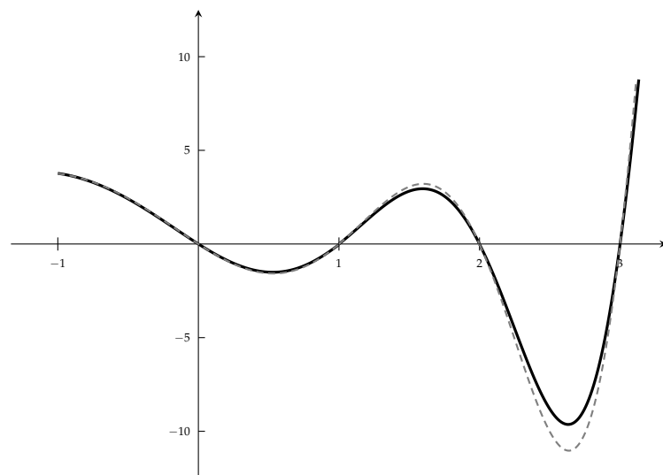
Figure 2. The gray color curve represents the function in the left hand side in (54) for n = 70 and black curve is the limiting function. Data: \beta = 7, c = 1/5, \lambda = 10^{-21} and j = 2 .
